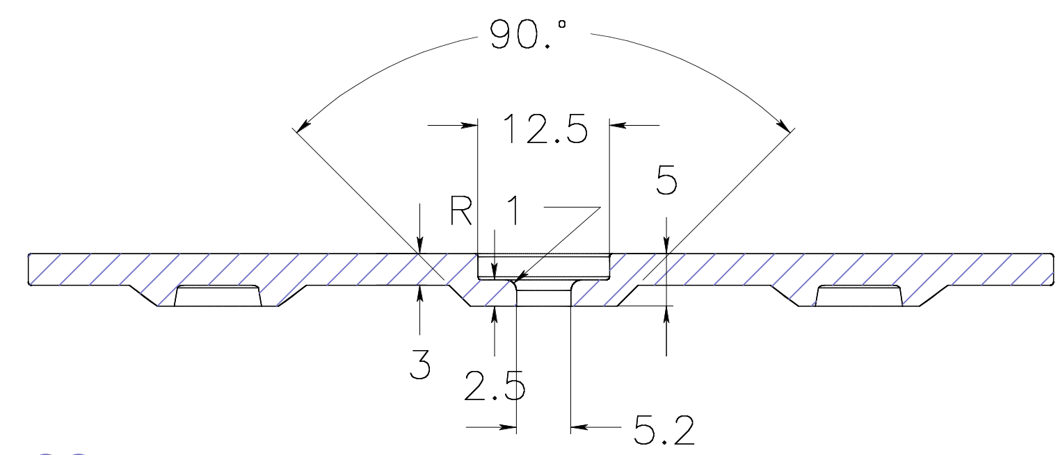
section GG
