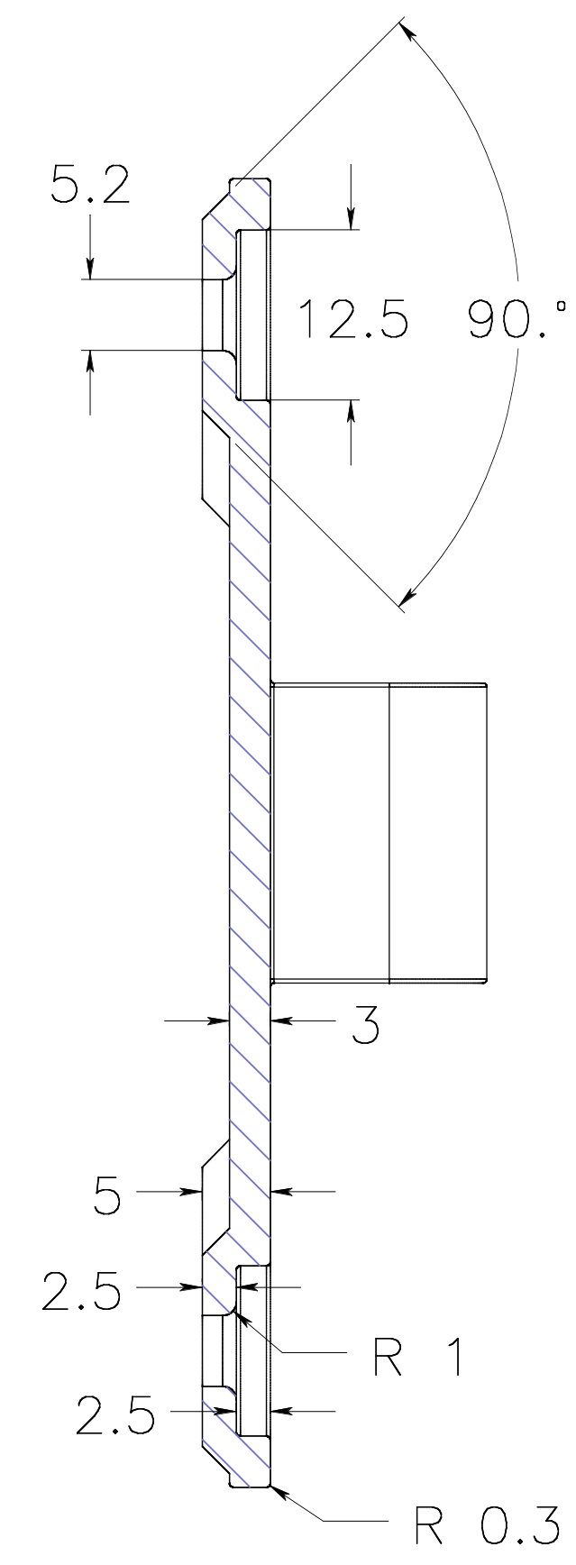
section CC
