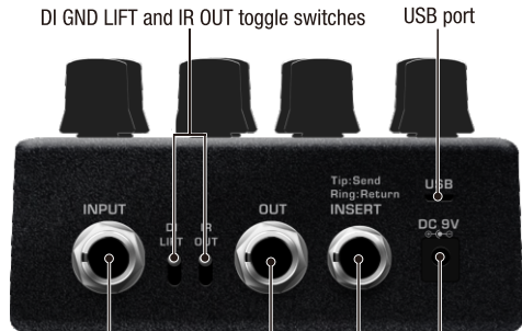
INPUT jack OUTPUT jack INSERT jack DC jack
